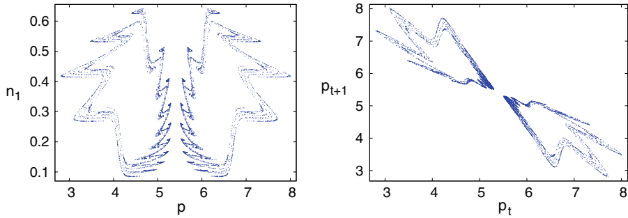
Fig. 6 Phase plot (left panel) with a strange attractor in the (p, n_1) plane. The same attractor shown in a delay plot (p_t, p_{t+1}) (right panel). Parameters are: \beta = 15, a = 10, b = 0.5, s = 1.35, C = 1, w = 0 and \delta = 0.8
