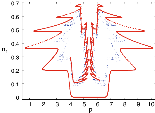
Fig. 7 Approximation of the unstable manifold of the steady state; 1, 000 point of the strange attractor are also shown. The approximation of the unstable manifold has been obtained by 19 iterations of 1, 000 initial states on a small vector with endpoints (p^*, 0) and (p^* + 0.001, 0) . Parameters are: \beta = 15, a = 10, b = 0.5, s = 1.35, C = 1, w = 0, \delta = 0.8 and p^* = a/(b + s) \approx 5.4054
