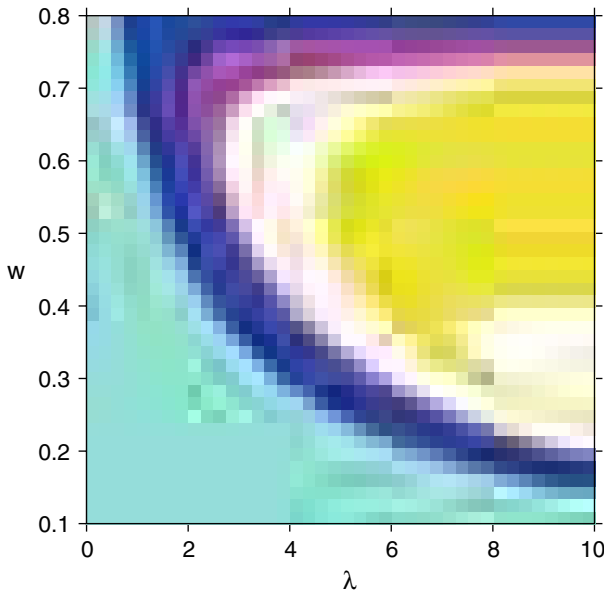
Fig. 3 Parameter Basins of stable steady state (light blue) and stable cycles of periods 2 (dark blue), 4 (purple), 8 (green), 3 (yellow), 5 (orange) and 7 (red), for 0 \leq \lambda \leq 10 and 0.1 \leq w \leq 0.8 with other parameters fixed at a = 1 and b = 0.25 and initial state x_0 = 0.3 . Transient iterations 500, resolution 450 \times 450 and convergence distance epsilon 0.001. Computation time 165 s (Pentium 3 GHz)
