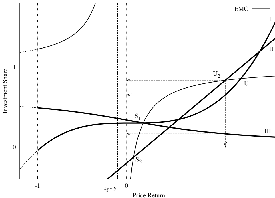
Figure 1: The intersections of the EMC and different investment functions illustrate the equilibria of system (2.8). Each of points S_2 , U_1 and U_2 define one equilibrium with one survivor. Point S_1 , instead, defines infinitely many equilibria with two survivors.
