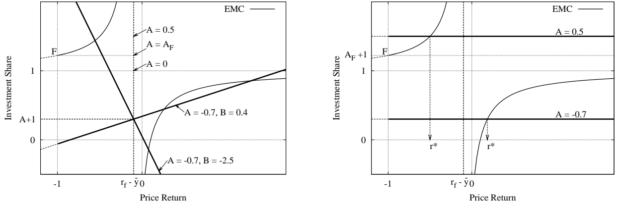
Figure 2: Left Panel: Examples of the linear investment functions (3.4) for different parameter pairs (A, B) . Right Panel: Equilibria for constant investment functions.
