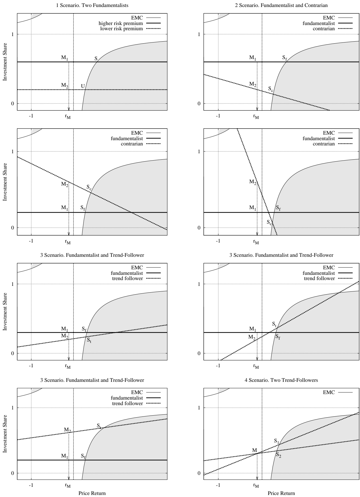
Figure 9: Equilibria in the model of Chiarella and He with two agents. See text for explanation.
