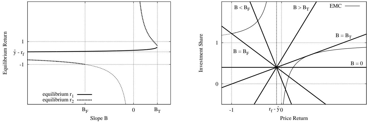
Figure 3: Equilibria r_1^* and r_2^* computed in Proposition 3.2 as functions of the slope B of the linear investment function for A = -0.6 ( left panel ), and their movement as a result of the rotation of the investment function on the EMC plot ( right panel ).
