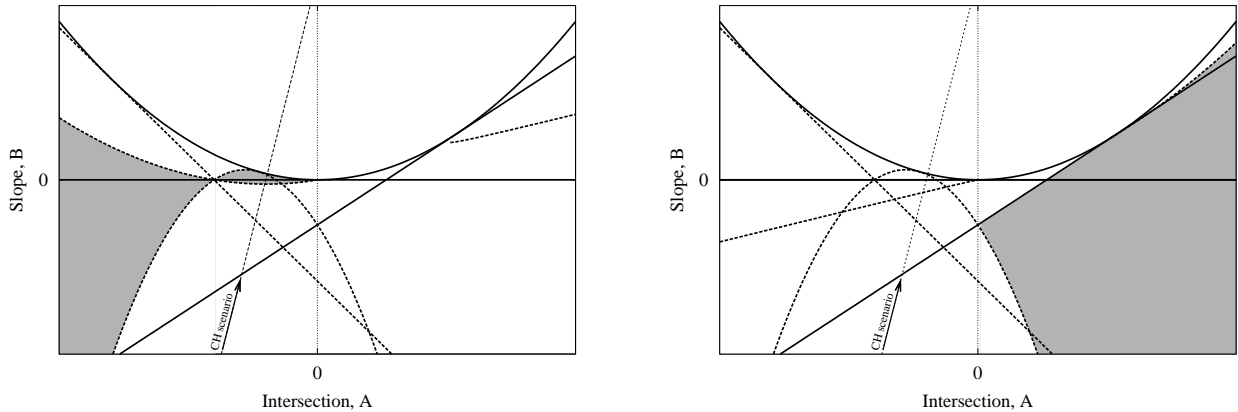
Figure 8: Stratification of the parameter space (A, B) according to the stability of equilibria. Left panel: stability of the first root r_1^* . Right panels: stability of the second root r_2^* . Corresponding root is stable if parameters belong to the grey area.
