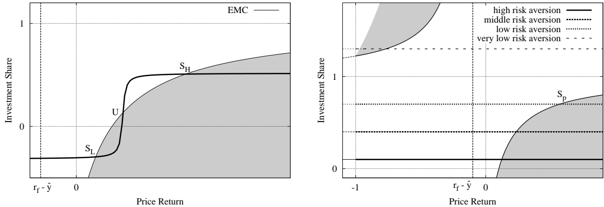
Figure 7: Left panel: In the market with single agent multiple stable equilibria can be generated by non-linear investment function. Right panel: Equilibria in the market with the EU maximizing fundamentalists.
