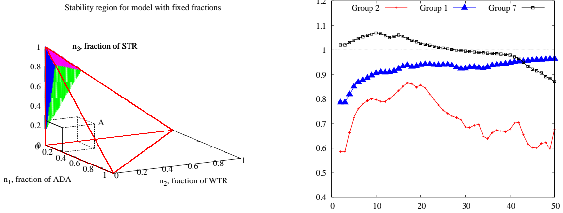
Figure 3: Local stability of fundamental steady-state in the constant weights model. Left: The fundamental steady-state is unstable in a model with four heuristics, when fixed weights (n_1, n_2, n_3) belong to the dark conic region of the unit simplex. Right: Evolution of the modulus of the largest eigenvalue of polynomial (14) corresponding to the simulations of the evolutionary model in Figs. 1 and 2.
