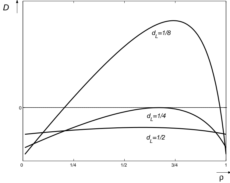
Figure 1: The difference in social welfare ( d_H = 1 and \gamma = 1 )
