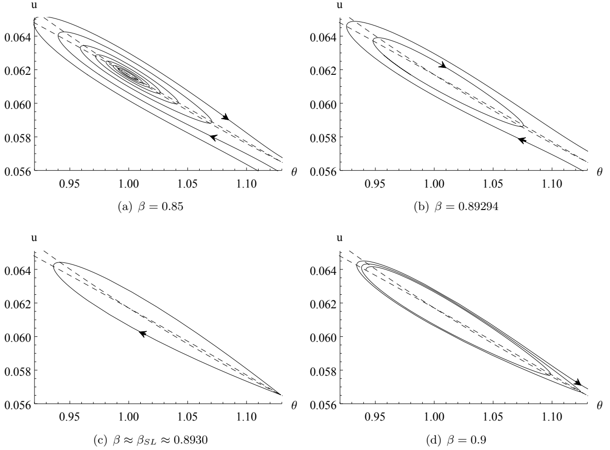
Figure 3: Representative phase diagrams for different values for \beta : (a) Stable steady state; (b) Stable limit cycle; (c) Homoclinic orbit of the saddle-loop bifurcation; (d) No closed orbits at efficient bargaining.
