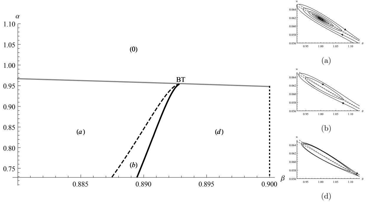
Figure 4: Bifurcation diagram of the Bogdanov-Takens bifurcation, with \alpha and \beta as bifurcation parameters. Notes: Other parameters from Table 3, first column. The gray curve corresponds to the saddle-node bifurcation, the bold curve to the saddle-loop bifurcation, and the dashed curve to the Hopf bifurcation. Regions (a), (b), and (d) refer to the panels of Figure 3, reprinted for convenience, and (d) extends beyond efficient bargaining at \beta = 0.9 (dotted curve). BT refers to the Bogdanov-Takens-point, and there are no steady states with economic activity in region (0). The homoclinic orbit hits the u -axis for \alpha \approx 0.73 .
