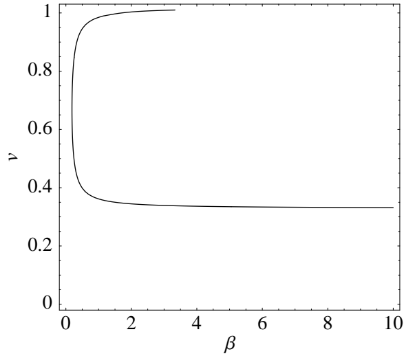
Figure 2: Plot of the curve DH of Chenciner bifurcation points lying within the Hopf bifurcation set H = \{g = 2R\} in the \beta - v -diagram, for \beta \in [0, 10] , v \in [0, 1] and R = 1.01 and \alpha = 1 fixed.
